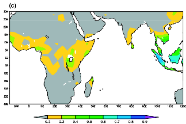
Figure 83: Theoretical limit of predictability, R_{limit} for September-to-November mean precipitation derived from an AGCM ensemble. From paper: Bahaga et al., 2015: Potential predictability of the sea-surface forced Equatorial East African short rains interannual variability in the 20th century. Q. J. R. Meteorol. Soc. , 141 , 16-26, doi: 10.1002/qj2338.
