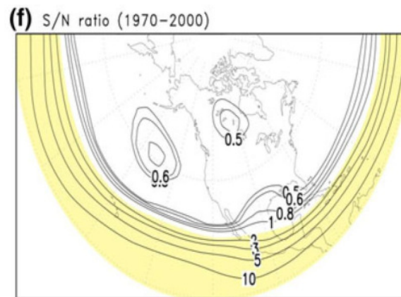
Figure 82: Signal-to-Noise ratio for winter (December-to-February) mean derived from an AGCM ensemble. Upper panel: Precipitation, lower pane: 200 hPa geopotential height. From paper: Ehsan et al., 2013: A quantitative assessment of changes in seasonal potential predictability for the 20th century. Clim Dyn , 41 , 2697-2709, doi: 10.1007/s00382-013-1874-x.
