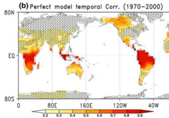
Figure 85: Potential Correlation Skill of near-surface temperature for winter (December-to-February) mean derived from an AGCM ensemble. From paper: Ehsan et al., 2013: A quantitative assessment of changes in seasonal potential predictability for the 20th century. Clim Dyn , 41 , 2697-2709, doi: 10.1007/s00382-013-1874-x.
