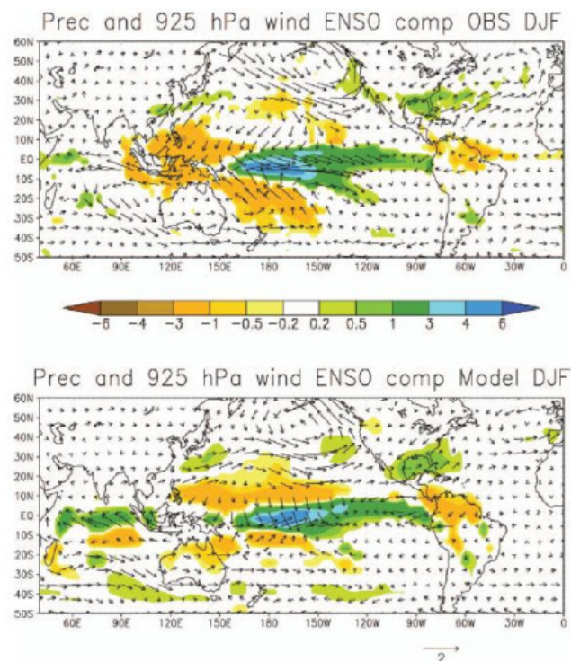
Figure 88: Regression coefficients b^* of the Niño3.4 index onto winter (December-to-February) mean precipitation. a) Observations, b) AGCM. Units are mm/day. From paper: Kucharski et al., 2015: On the need of intermediate complexity General Circulation Models: A “SPEEDY” Example. BAMS , 94 , 25-30, DOI: 10.1175/BAMS-D-11-00238.1.
