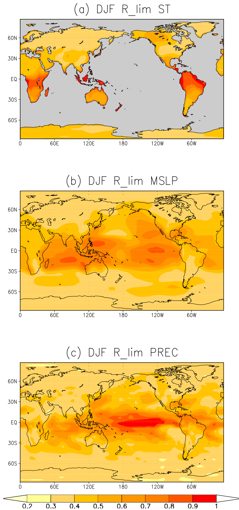
Figure 84: Theoretical limit of predictability, R_{limit} for December-to-February mean a) surface temperature, b) mean sea level pressure and c) precipitation for the DJF season derived from an AGCM ensemble. From Thesis: Bianca Mezzina, 2016: Seasonal influences of SST variability on European climate. University of Trieste Master thesis.
