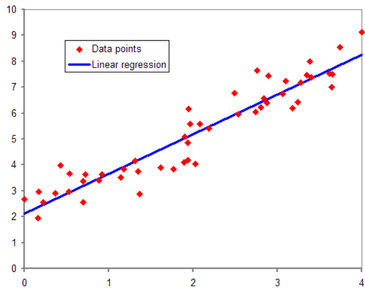
Figure 87: Linear regression method.
